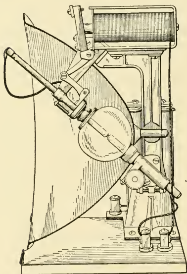
Fig. 116. Section of Arc Headlight
